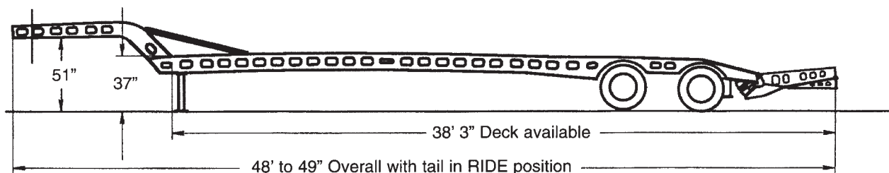
Model CSDF: Covered Tire, Single Drop, Fixed Gooseneck
