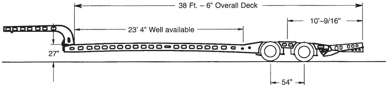
Model ODDF: Open Tire, Double Drop, Fixed Gooseneck
