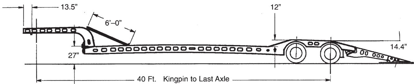
Model CDDD: Covered Tire, Double Drop, Detachable Gooseneck
